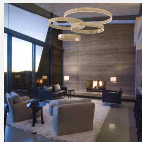
WIND UP (CLUSTER) DIMENSION - CLUSTER - Ø5'-0" X 5'-9" X 2'-2" H (4 ELEMENTS) MATERIAL - WOOD LIGHTING - LED
